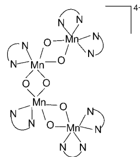
Figure 1. Schematic drawing of [\text{Mn}_4(\mu\text{-O})_6(\text{bipy})_6]^{4+} . N–N = 2,2'-bipyridine.
